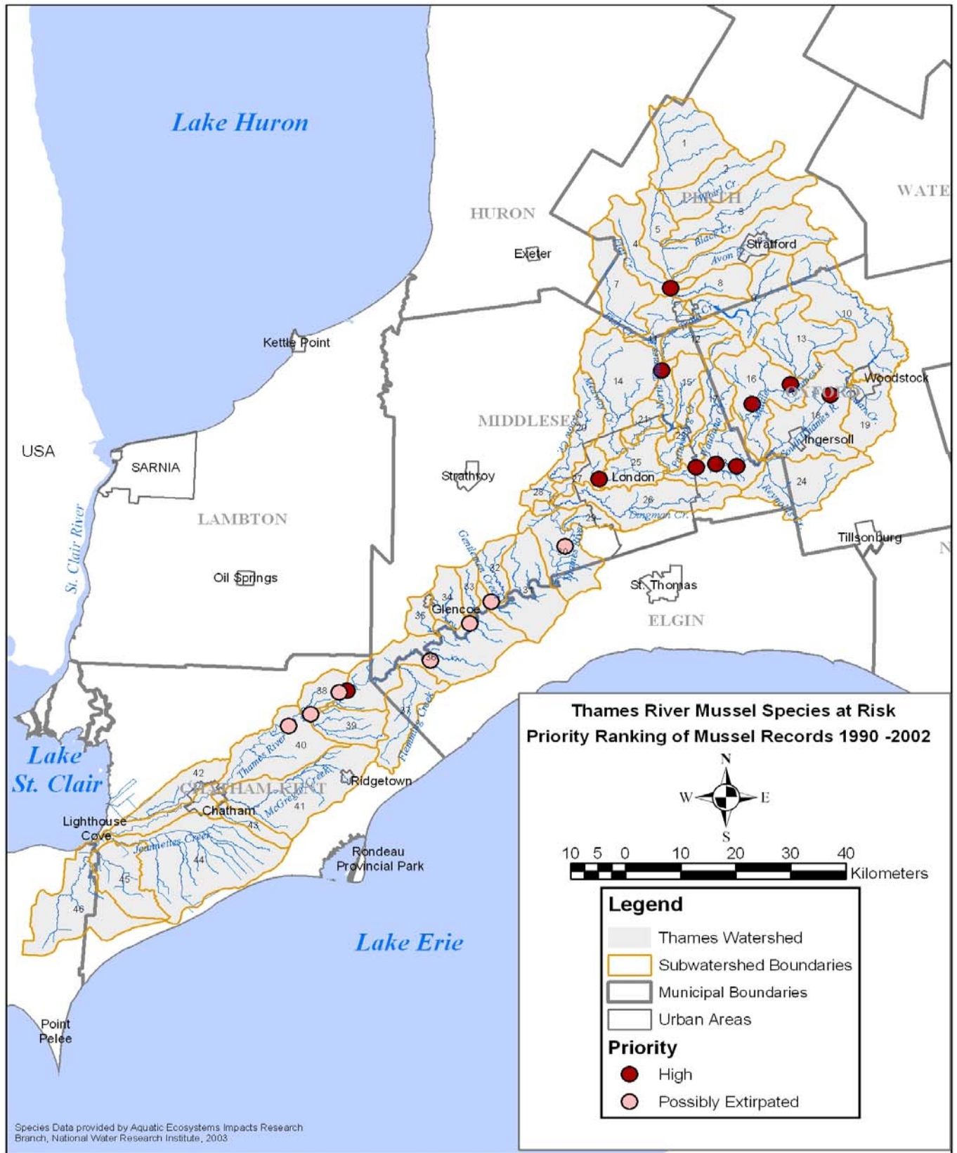
Figure 10. Mapping of recent (1990-2002) occurrence evidence of mussel species at risk by priority in the Thames River watershed.
