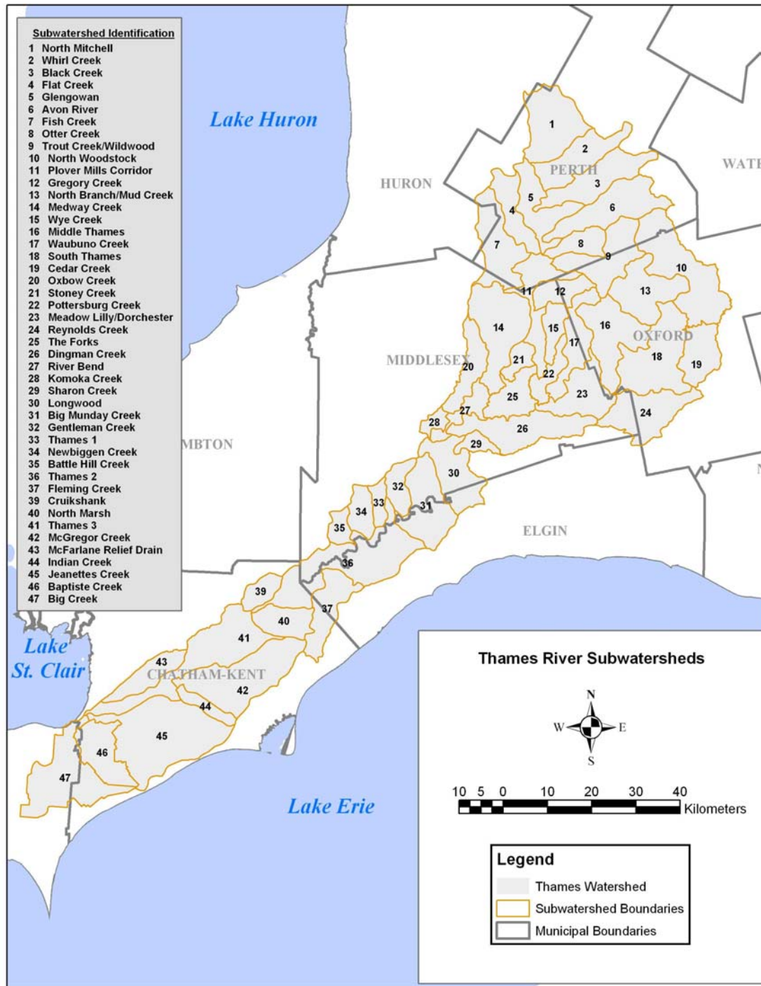
Figure 2. Subwatersheds of the Thames River watershed. For all other watershed maps contained in this report, numbered labels refer to these numbered subwatershed names.
