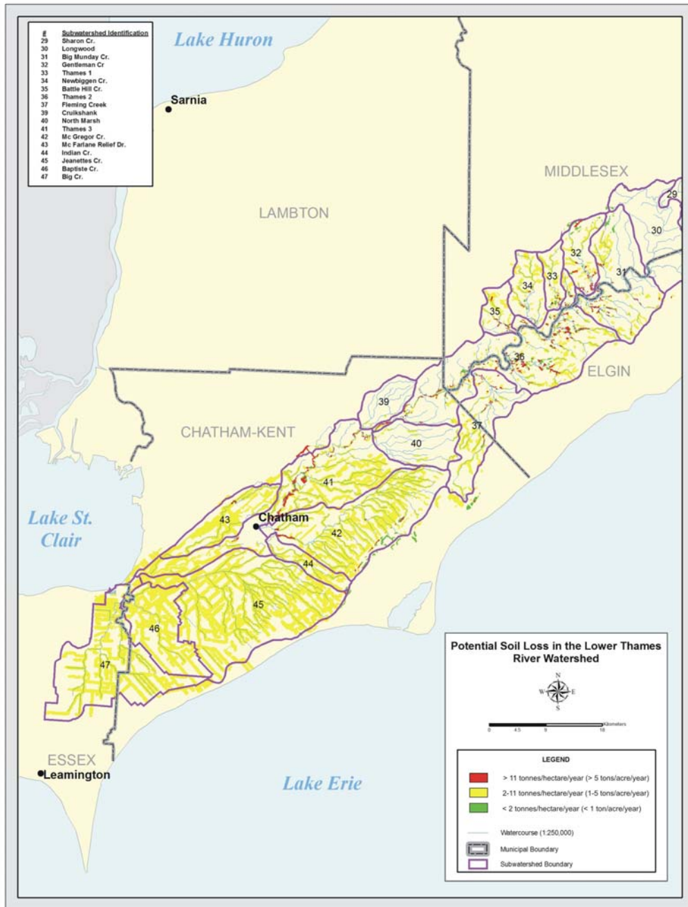
Figure 5. Potential soil loss (tonnes/hectare/year) in the lower Thames River watershed.
